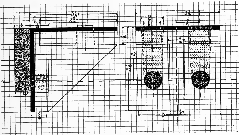
FIG. 523. PATTERN-MAKER'S LAY-OUT OR DRAWING.
